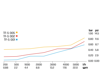
Pressure Loss
